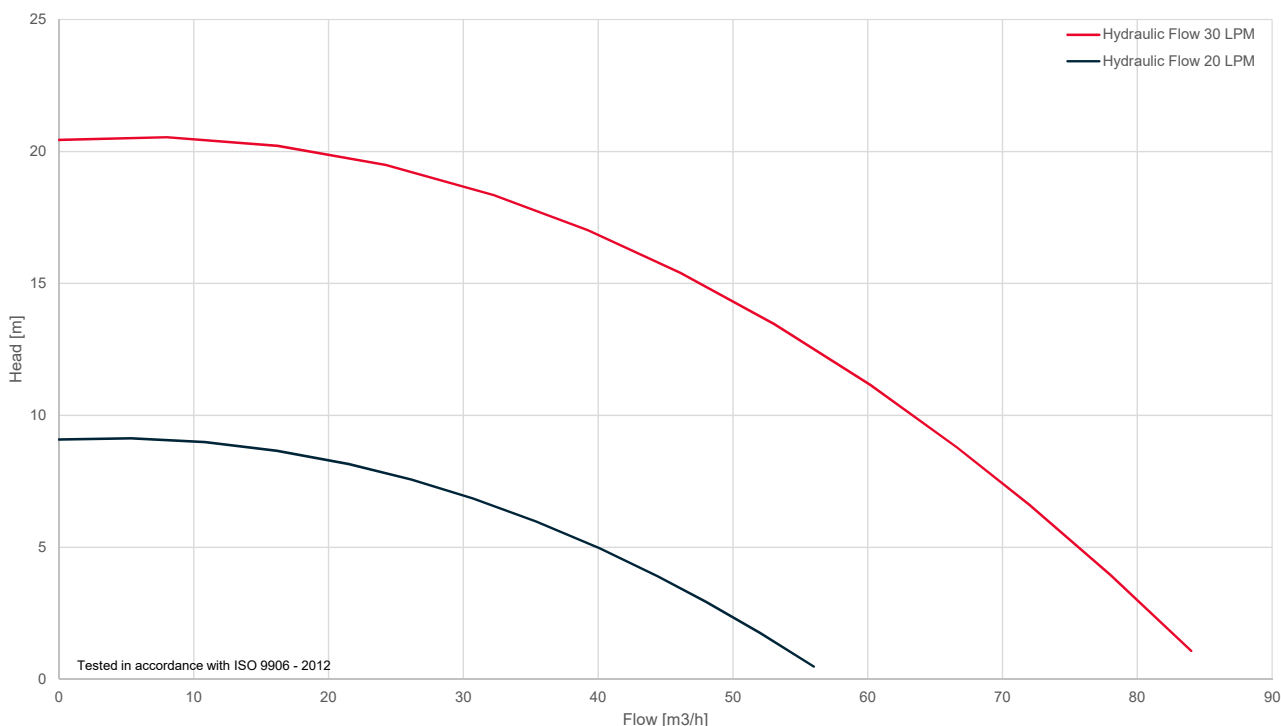
3" Submersible Pump
